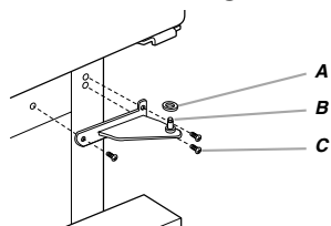
A. Shim (on some models) B. Center Hinge C. Hinge Screws
